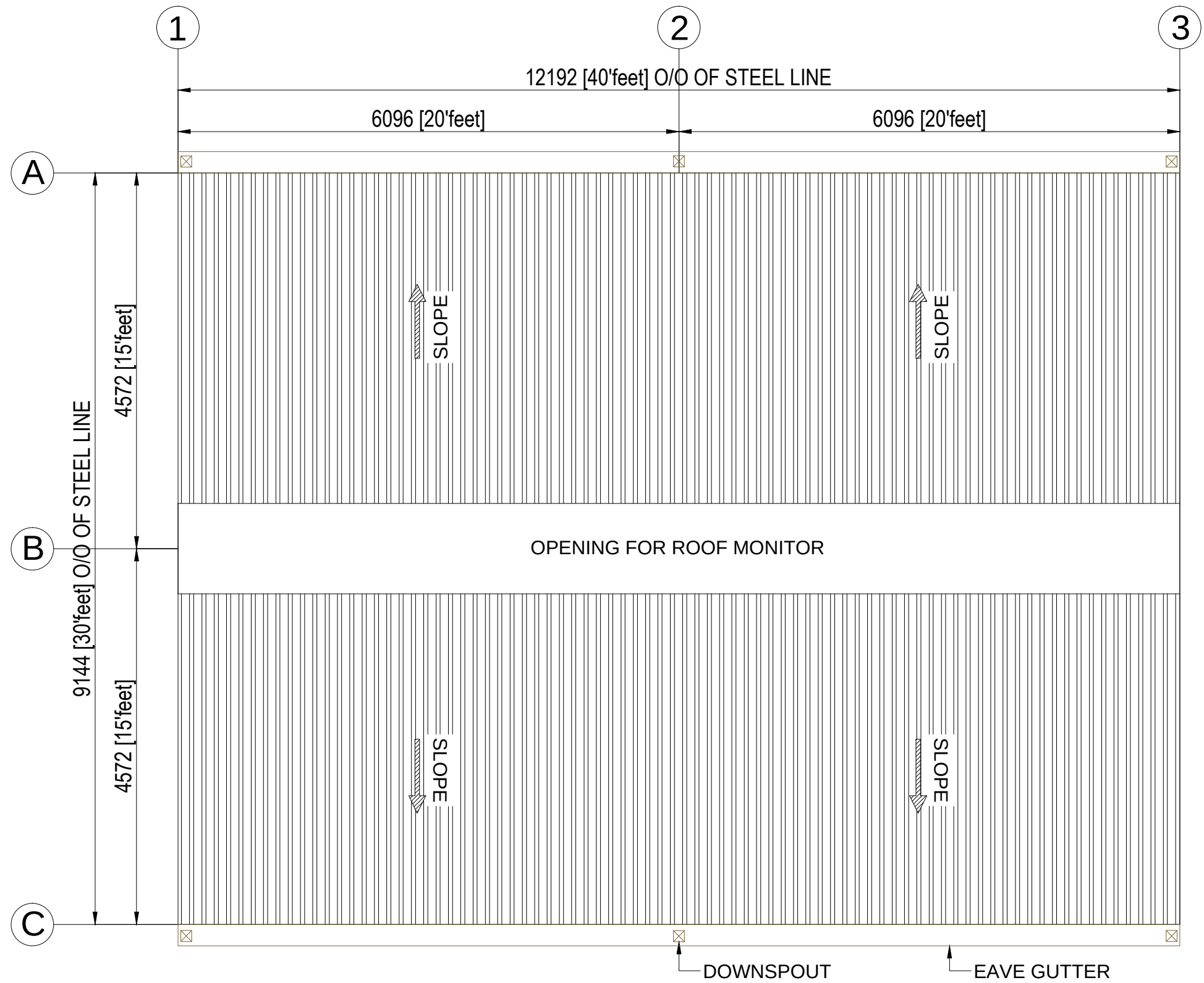
ROOF SHEETING PLAN
